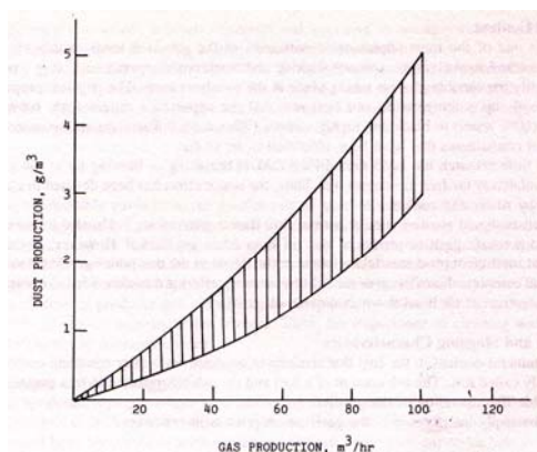
FIGURE 7. Dust content as a function of gas production.
